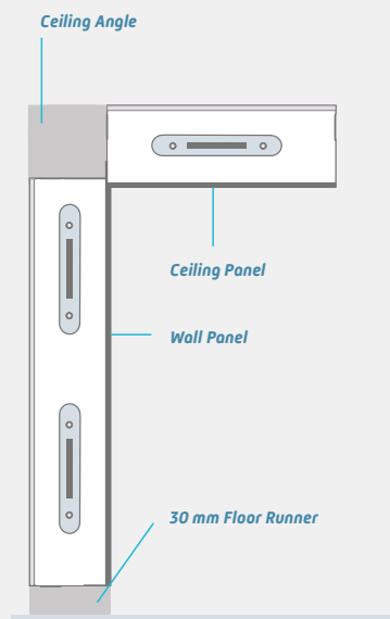
MATRIX 60, 85 and 105 - WITHOUT FLOOR
