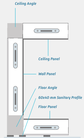
MATRIX 60, 85 and 105 - WITH FLOOR
