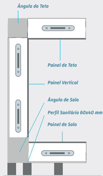
MATRIX 60, 85 e 105 - COM SOLO
