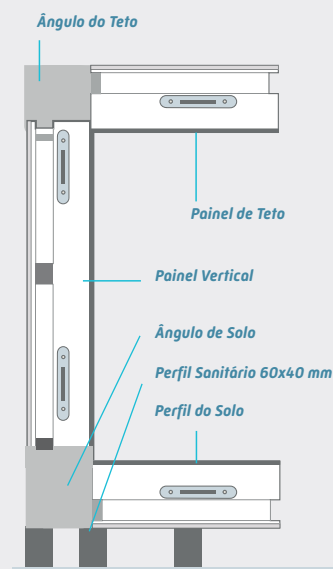
MATRIX 150 - COM SOLO
